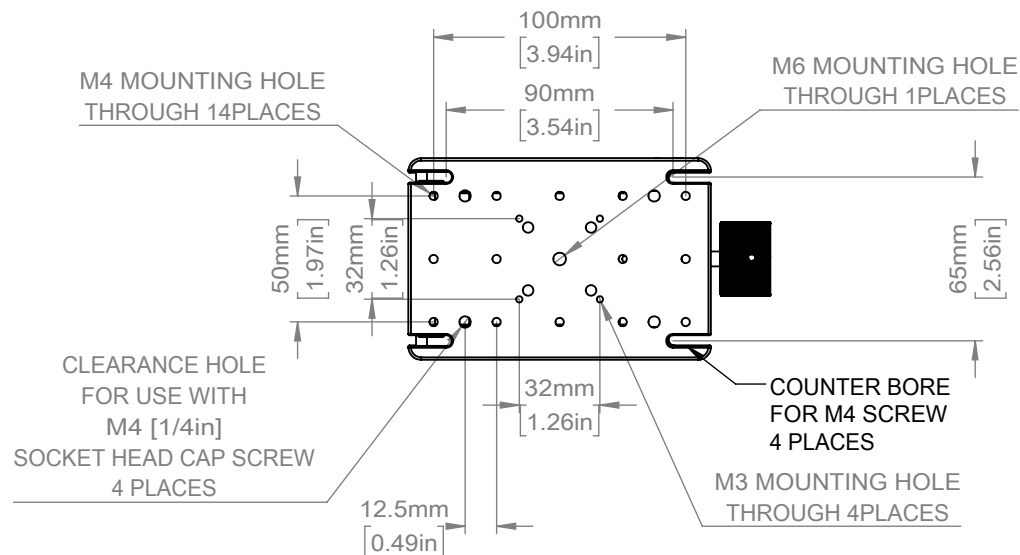
FULLY RETRACTED
