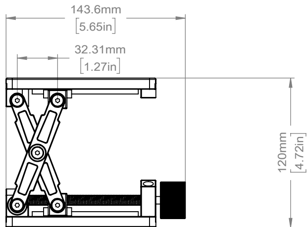
FULLY EXTENDED
