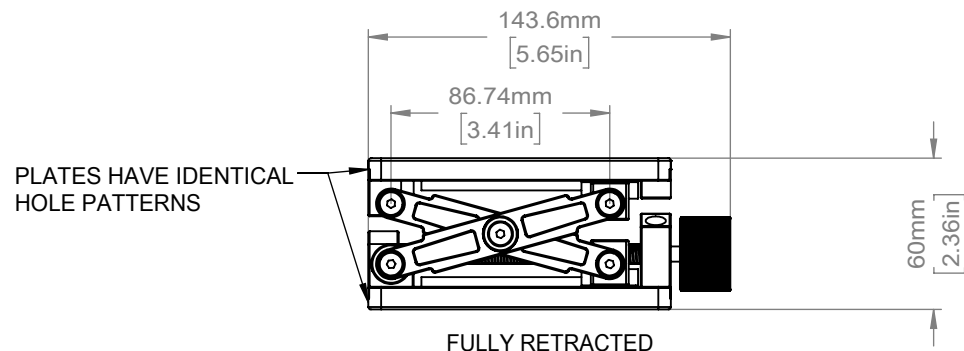
FULLY RETRACTED
